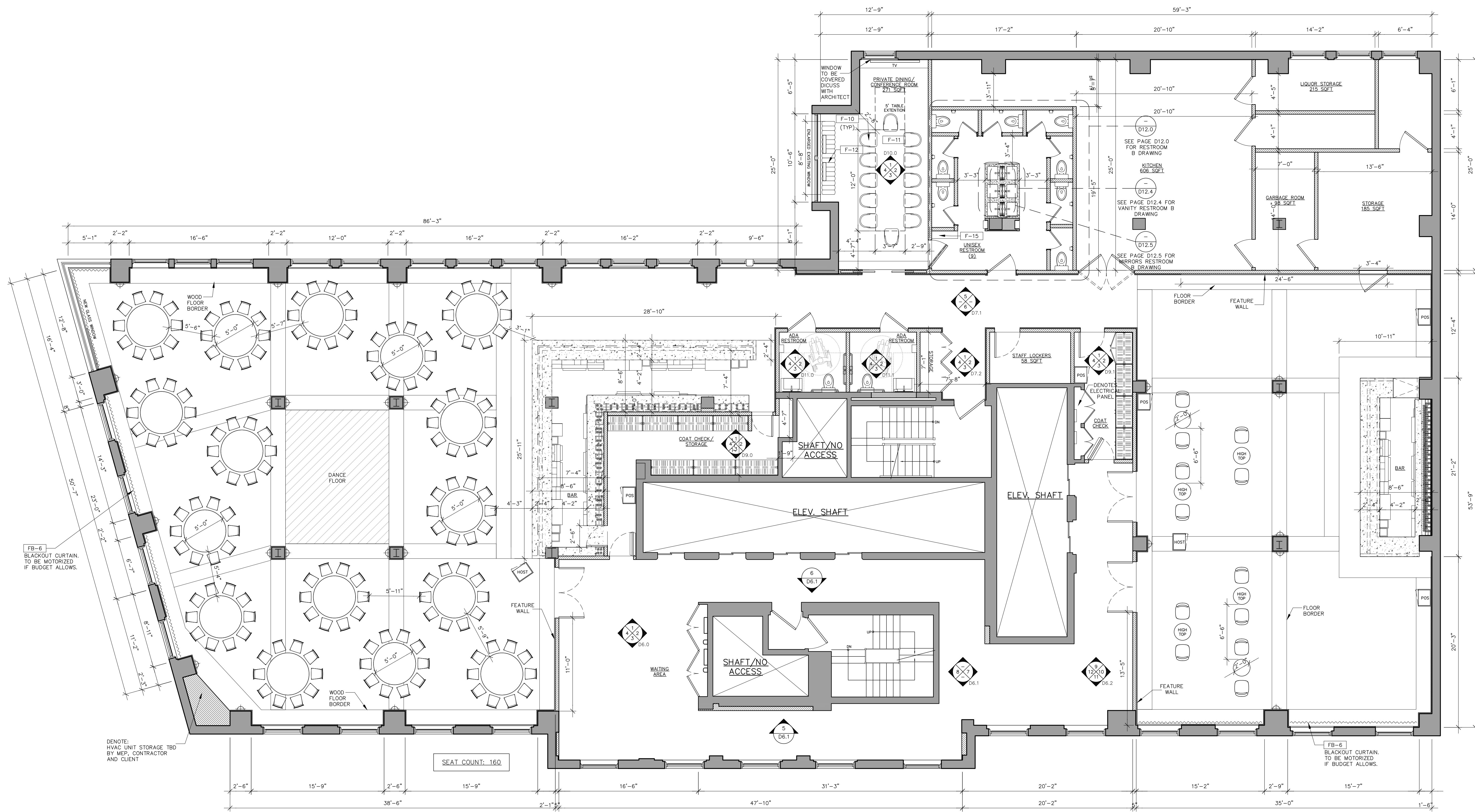
1 FURNITURE PLAN D1.1 SCALE: 3/16"=1'-0"
